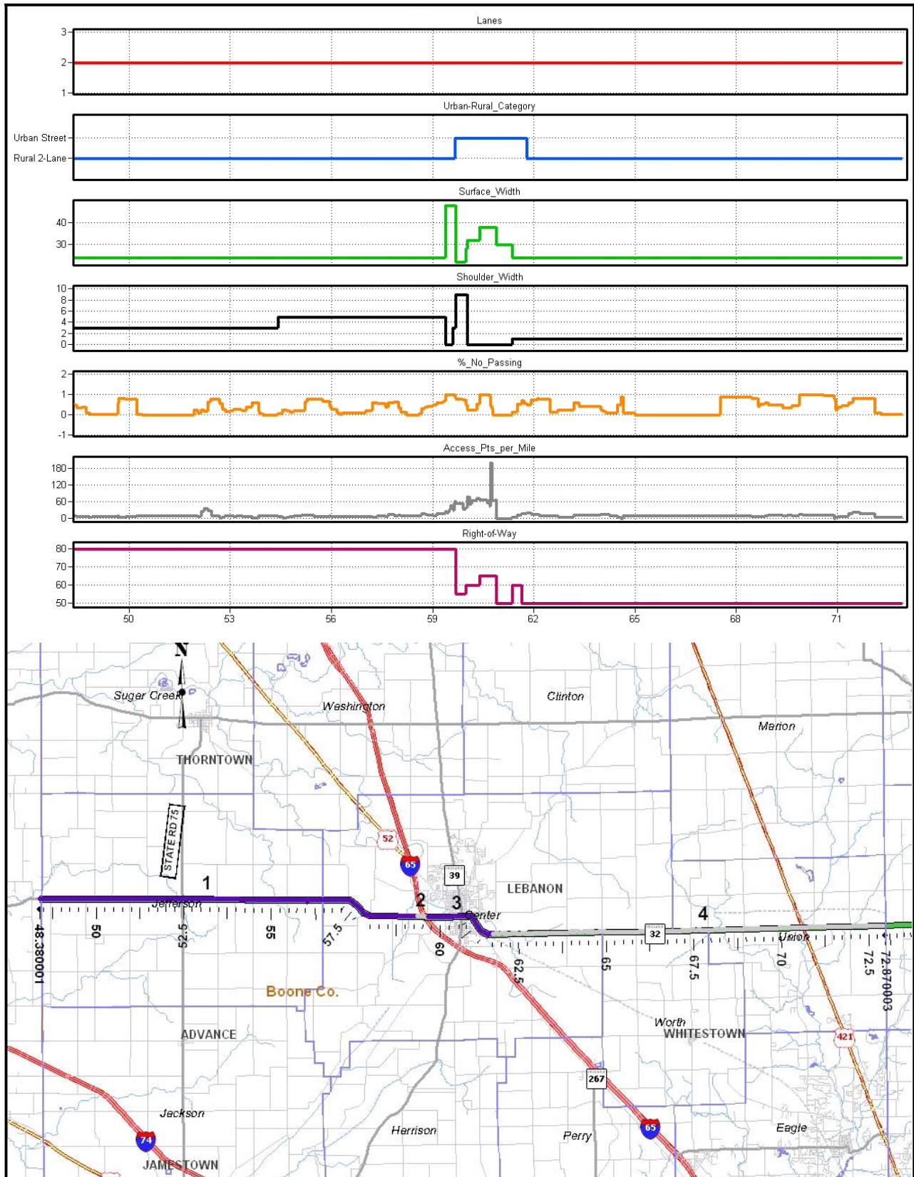
Figure 5-2: Physical Features - SR 32, Boone County
