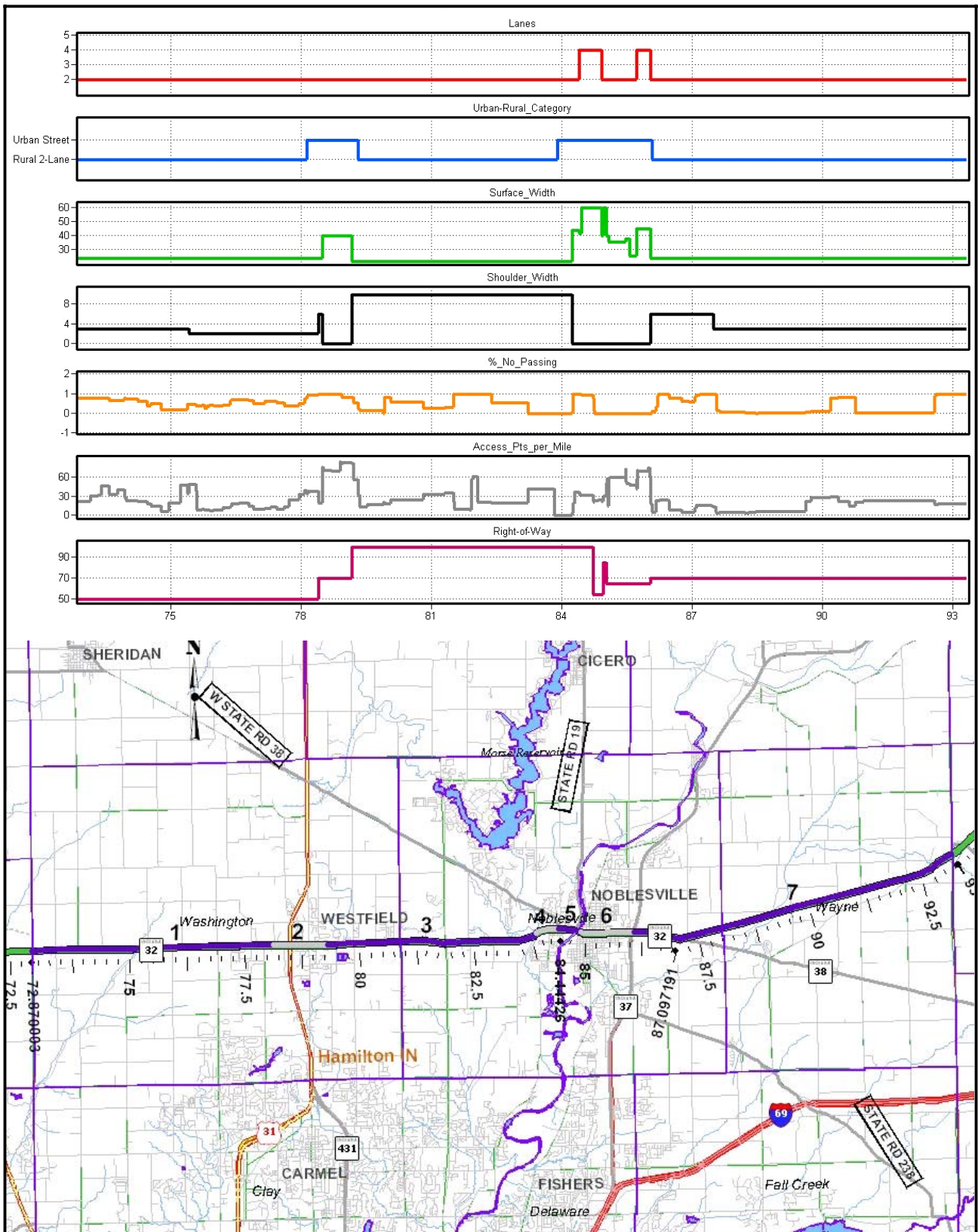
Figure 5-4: Physical Features - SR 32, Hamilton County
