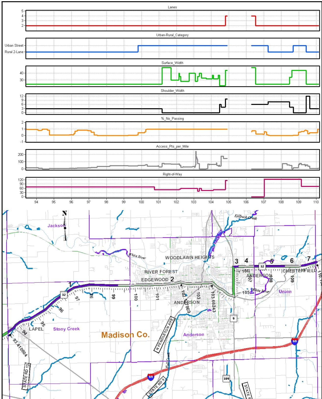
Figure 5-6: Physical Features – SR 32, Madison County
