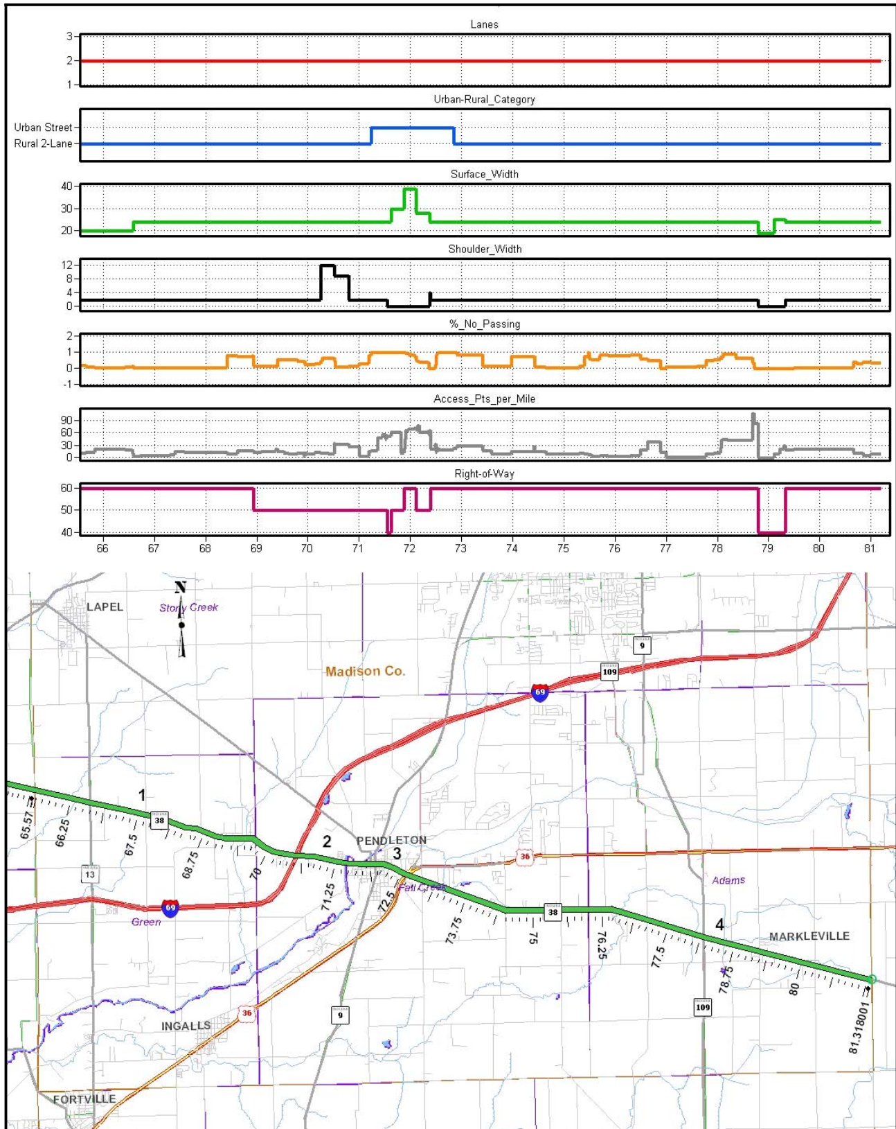
Figure 5-15: Physical Features – SR 38, Madison County
